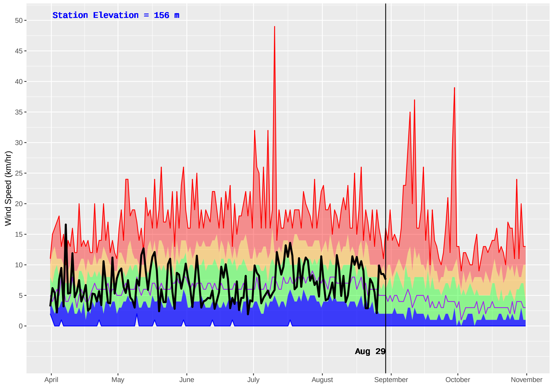
WOSS CAMP (21) : Historical (1970–2016) and Current (2018) Daily Wind Speed
