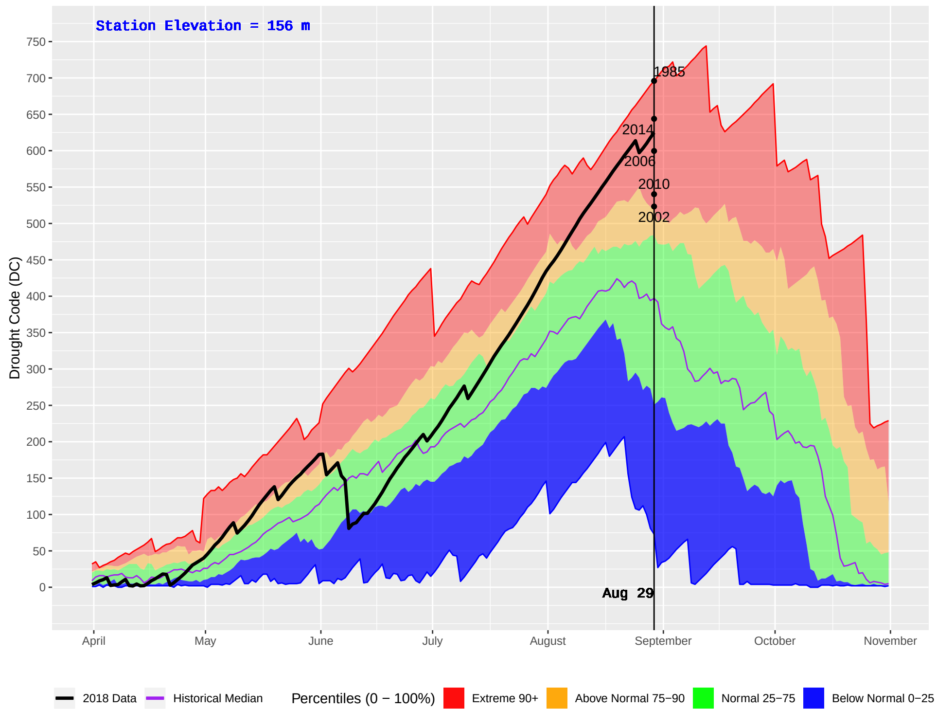
WOSS CAMP (21) : Historical (1970–2016) and Current (2018) Daily Drought Code (DC)
