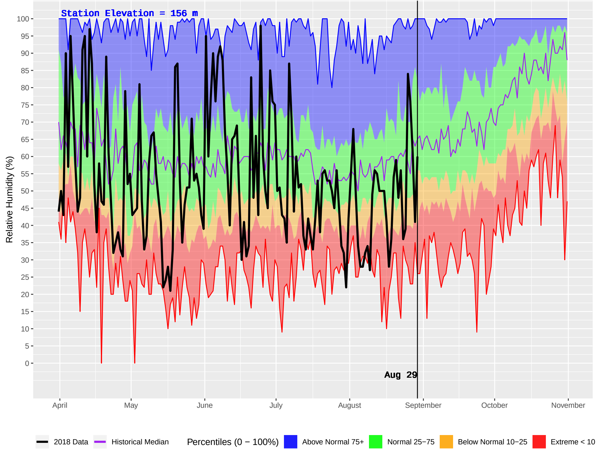
WOSS CAMP (21) : Historical (1970–2016) and Current (2018) Daily Relative Humidity
