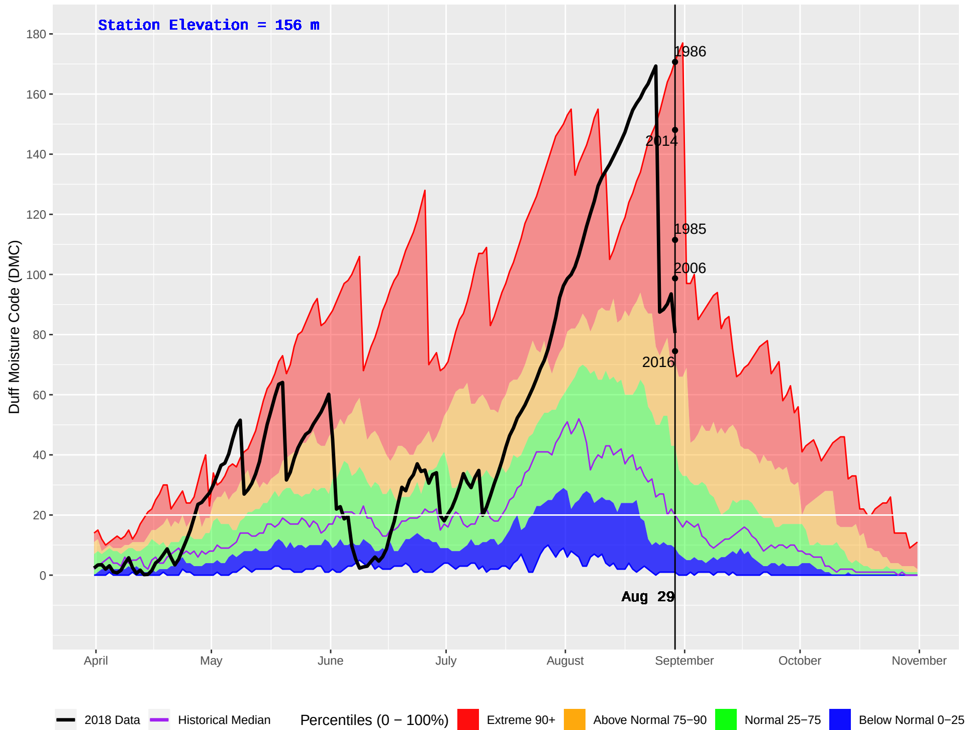
WOSS CAMP (21) : Historical (1970–2016) and Current (2018) Daily Duff Moisture Code (DMC)
