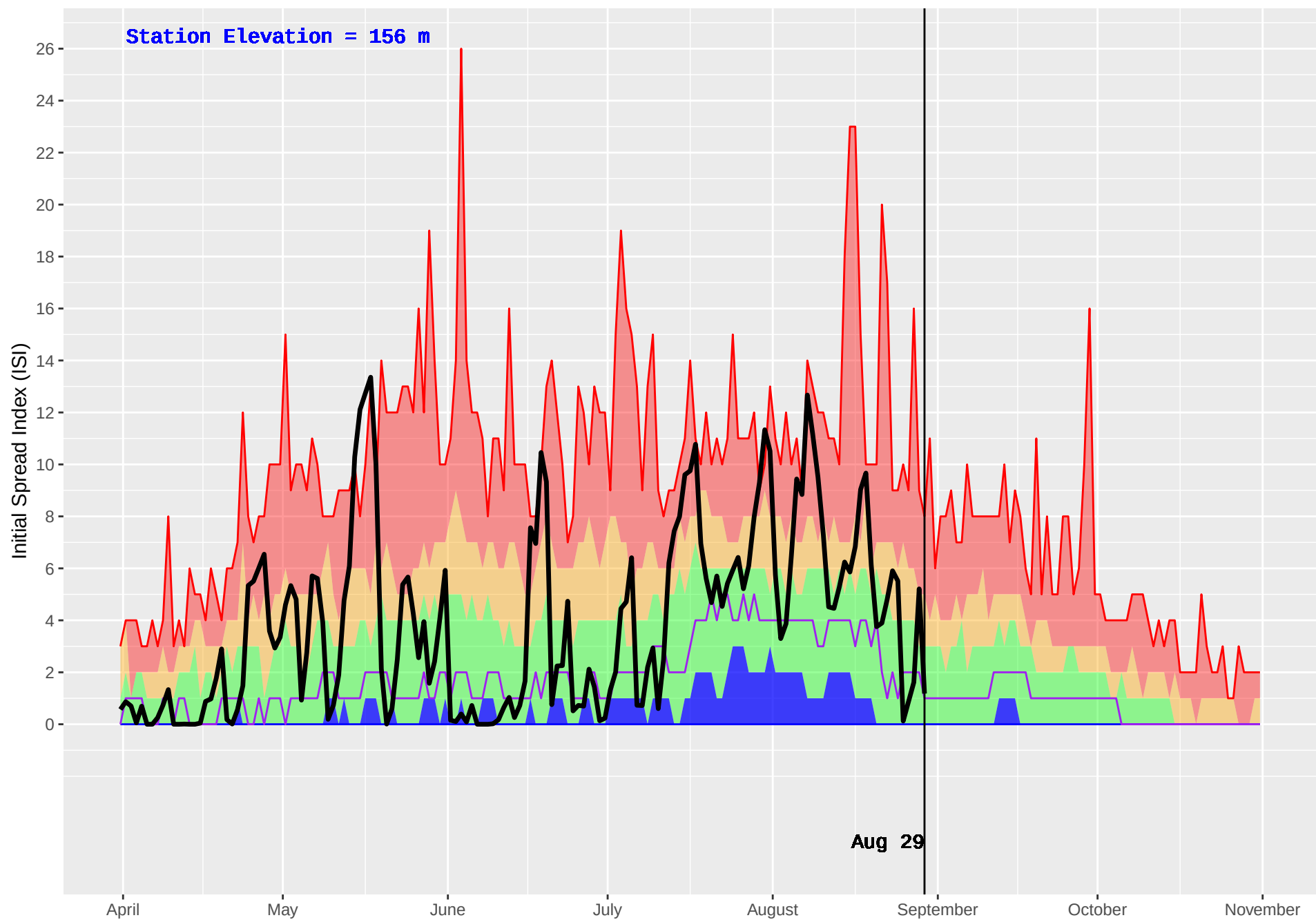
WOSS CAMP (21) : Historical (1970–2016) and Current (2018) Daily Initial Spread Index (ISI)
