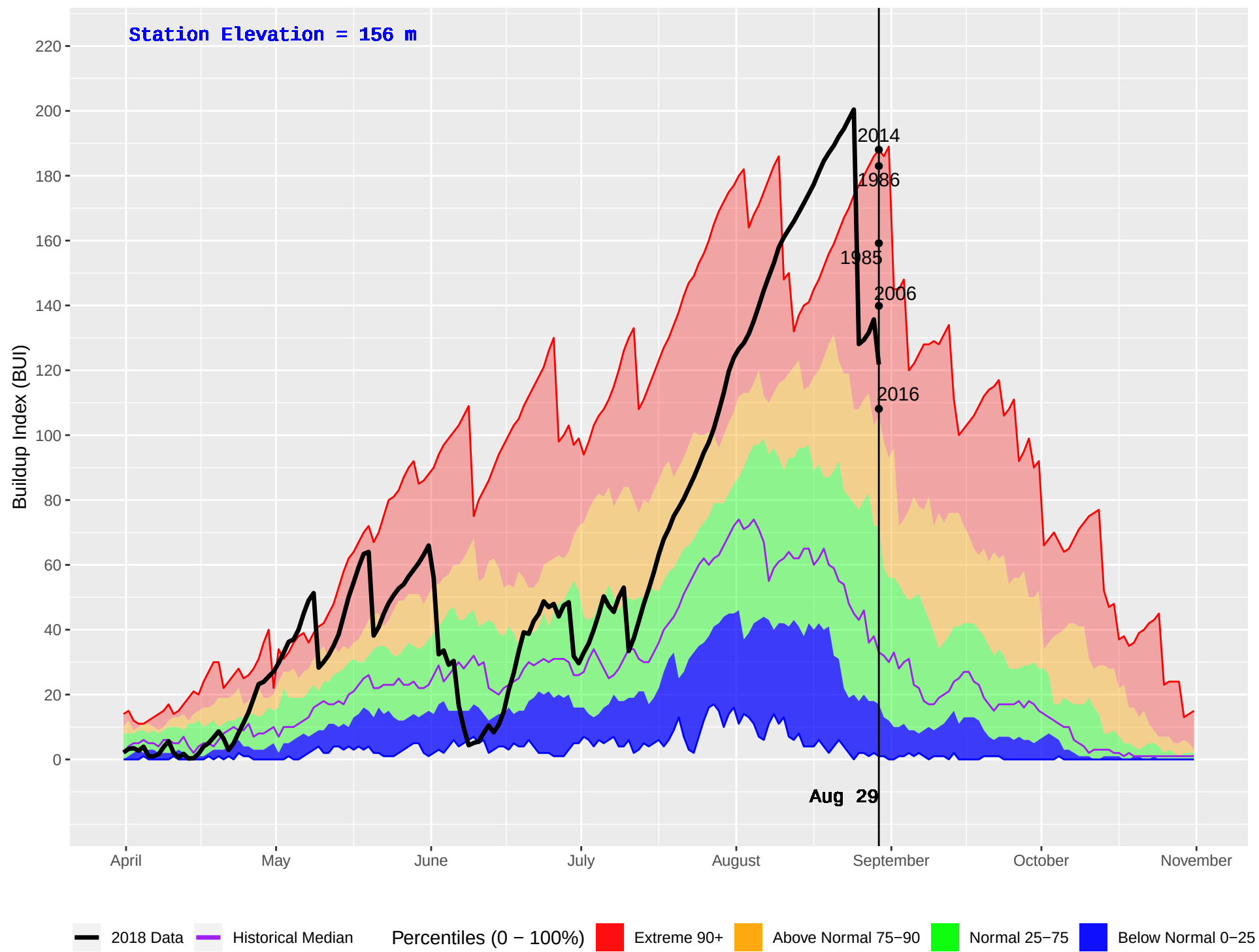
WOSS CAMP (21) : Historical (1970–2016) and Current (2018) Daily Buildup Index (BUI)
