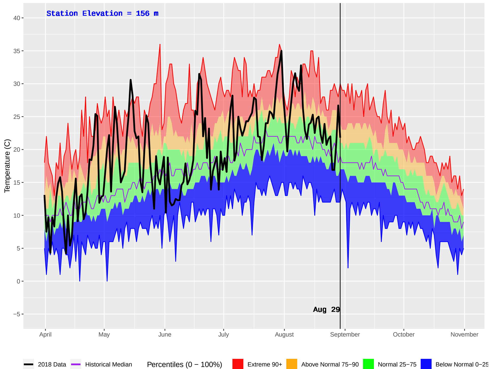
WOSS CAMP (21) : Historical (1970–2016) and Current (2018) Daily Temperature
